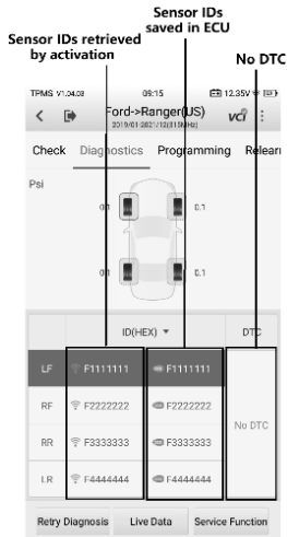
Figure 4-14 No DTC Screen
