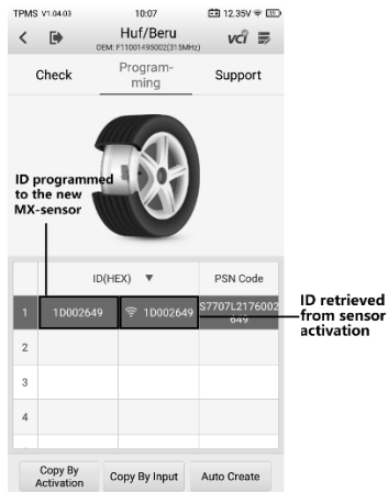
Figure 7-5 Programming Screen via OEM Part No.
