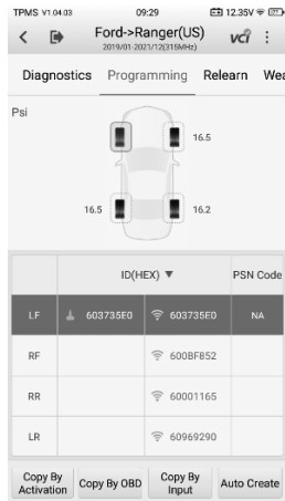
Figure 4-21 Copy by Activation Complete Screen
