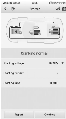
Figure 6-11 Starter Test Result Screen
