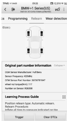
Figure 4-28 Automatic Relearn Screen 1
