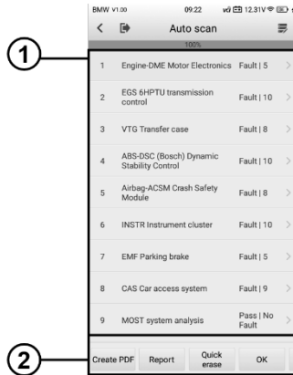
Figure 8-9 Auto Scan Operation Screen
