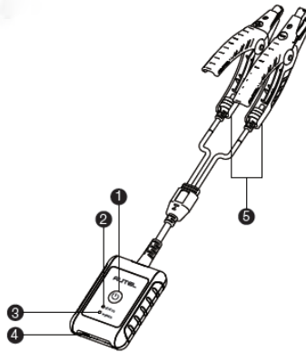
Figure 6-1 MaxiBAS BT506 Battery Tester
