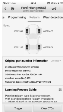
Figure 4-30 Stationary Relearn Screen 1
