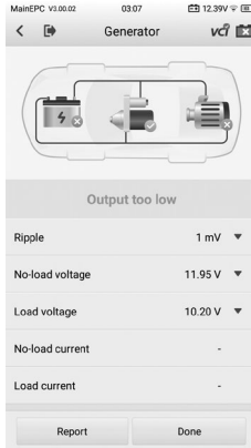
Figure 6-12 Generator Test Result Screen
