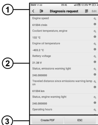
Figure 8-13 Live Data Screen
