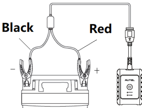
Figure 6-2 Connecting to a Battery
