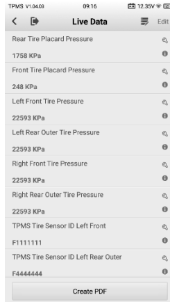
Figure 4-15 Live Data Screen
