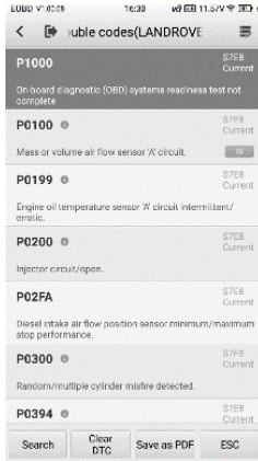
Figure 8-16 DTC & FFD Screen
