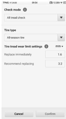
Figure 4-34 Check Settings Screen
